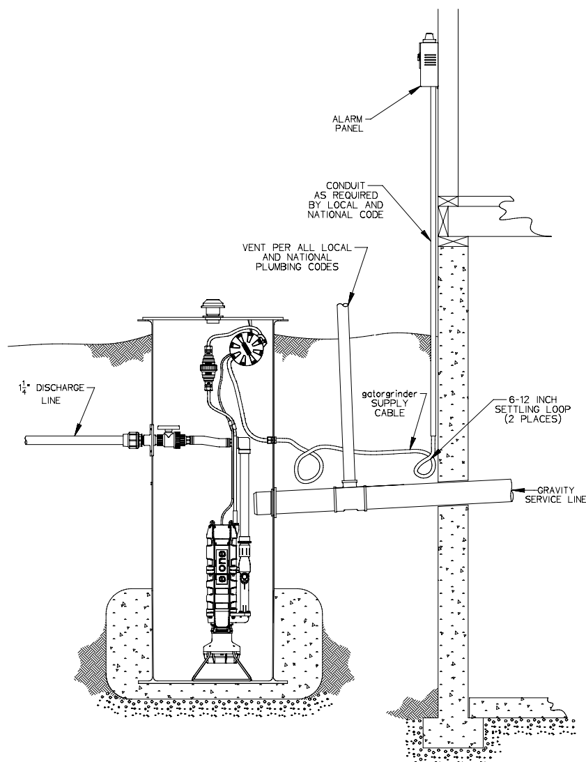
FIG. 5 - TYPICAL STATION INSTALLATION
